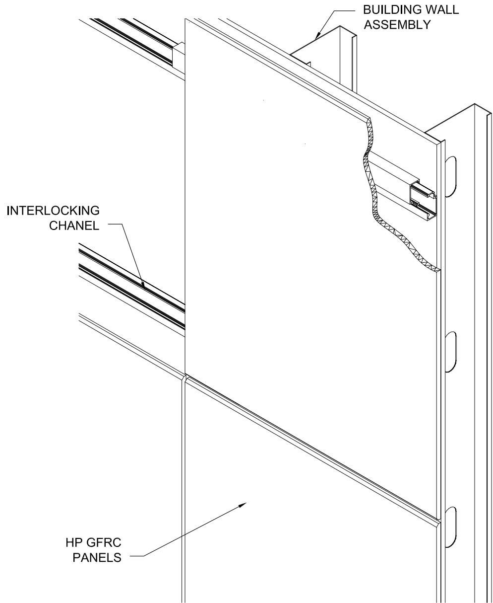
D1 INTERLOCKING PANELS NTS
