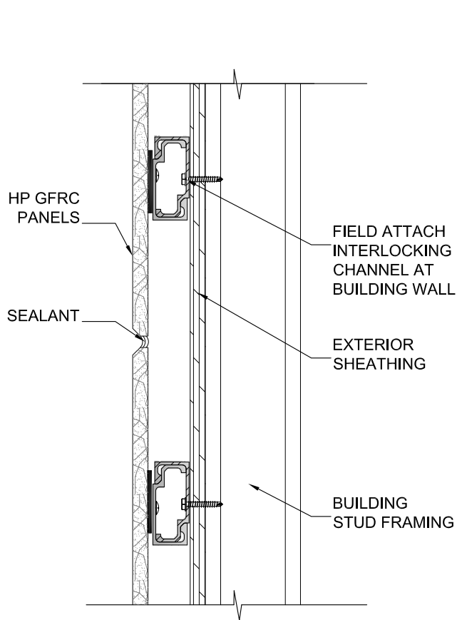
D2 WALL SECTION DETAIL NTS
